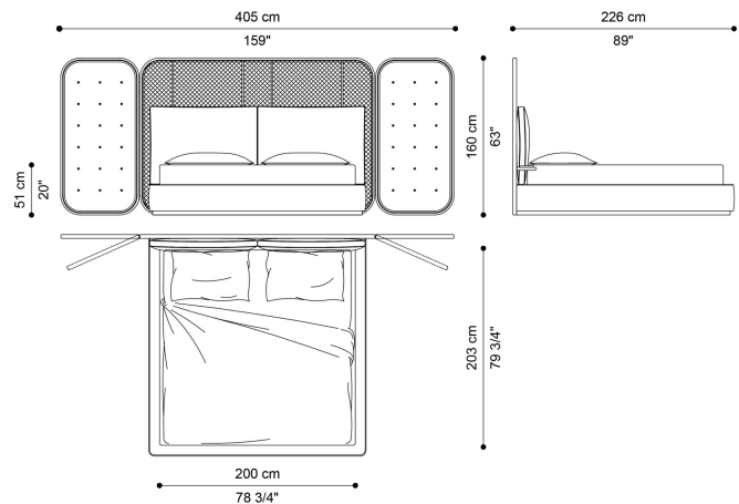
BED - FOR MATTRESS L 200 D 200 CM T.TIMBD01F
