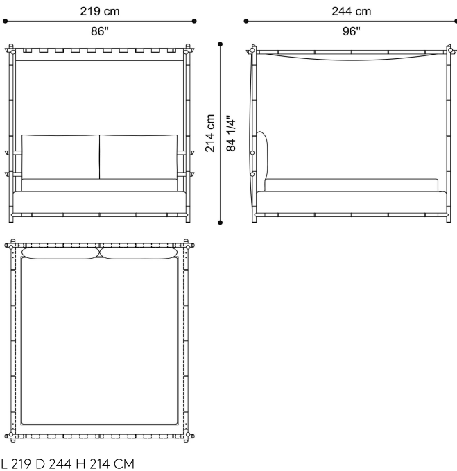
BED - WITH CANOPY - FOR MATTRESS 180 X 200 CM T.BLOBD04D
