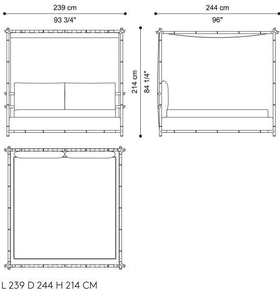
BED - WITH CANOPY - FOR MATTRESS 200 X 200 CM T.BLOBD04F
